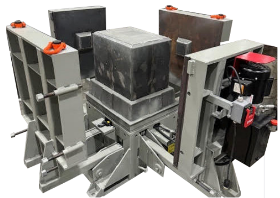
Small Four Roll Back Form
